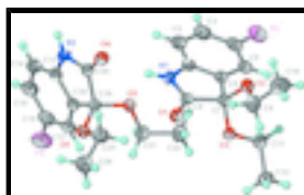
Fig. 1. Thermal ellipsoid plot (Barbour, 2001) of the two molecules of C_{12}H_{14}FNO_3 at the 70% probability level; hydrogen atoms are drawn as spheres of arbitrary radius.
